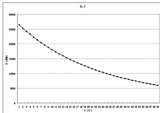
Temperature graph against resistance
